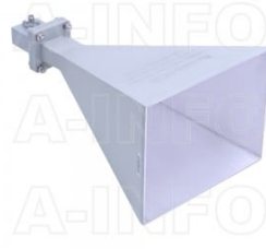
LB-90-20-C-SF Standard Gain Horn Antenna 8.2-12.4GHz 20dB Gain SMA Female
